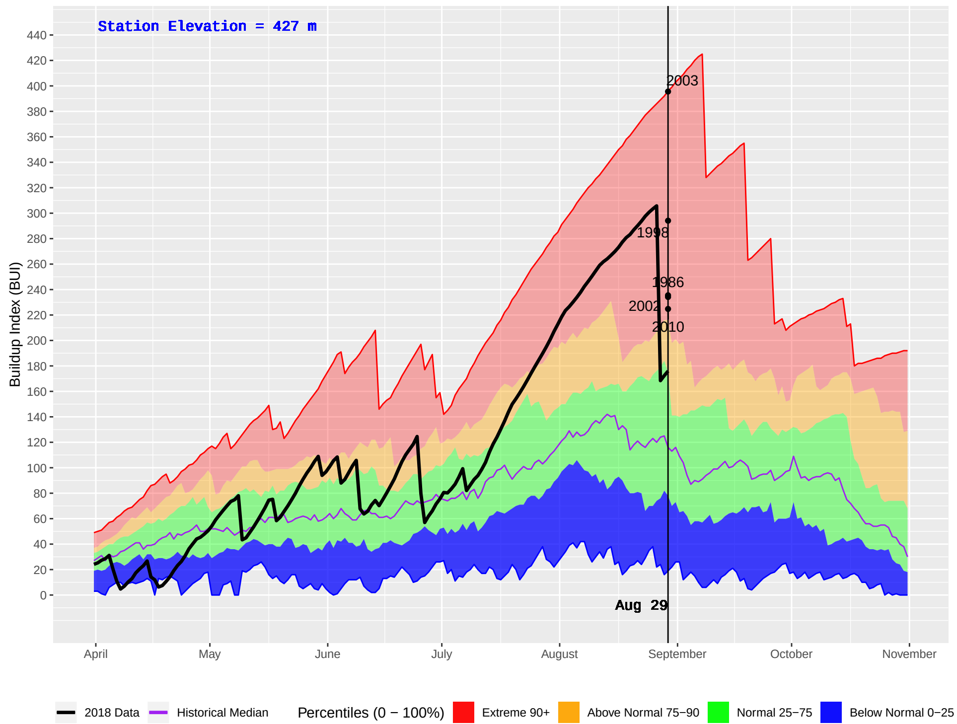
PENTICTON RS (328) : Historical (1970–2016) and Current (2018) Daily Buildup Index (BUI)
