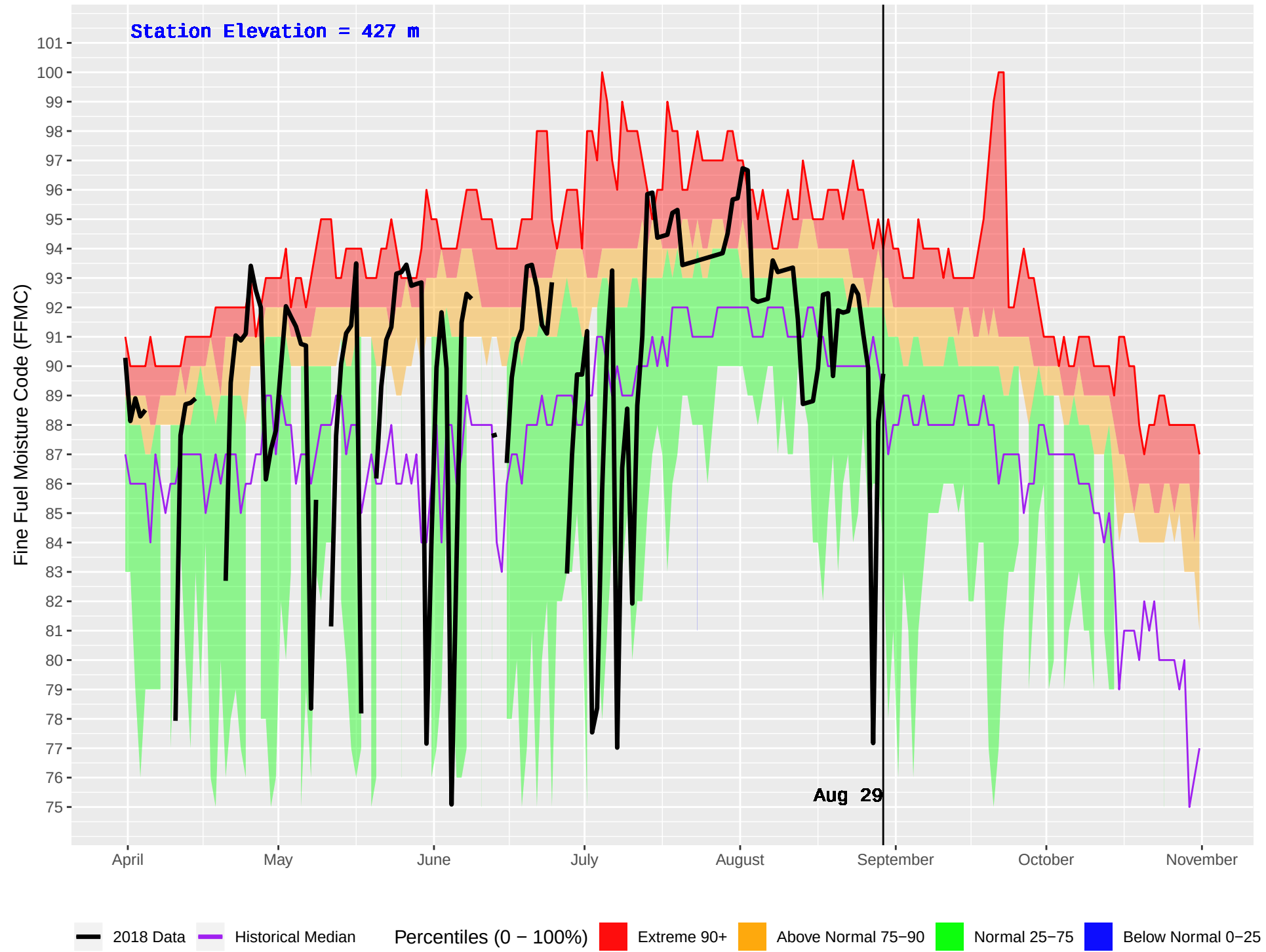
PENTICTON RS (328) : Historical (1970–2016) and Current (2018) Daily Fine Fuel Moisture Code (FFMC)
