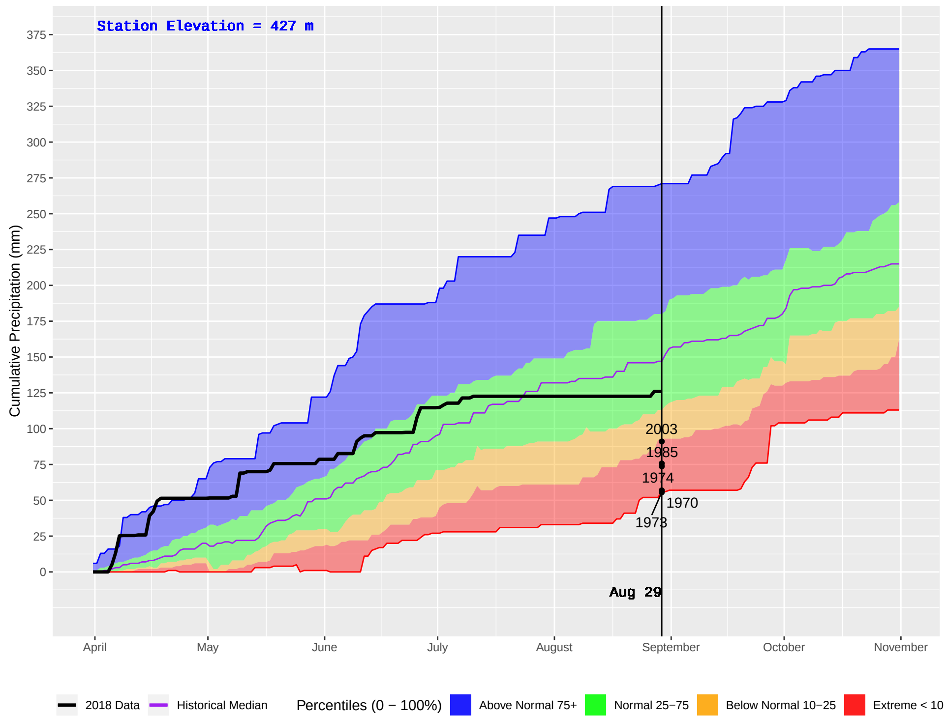
PENTICTON RS (328) : Historical (1970–2016) and Current (2018) Daily Cumulative Precipitation
