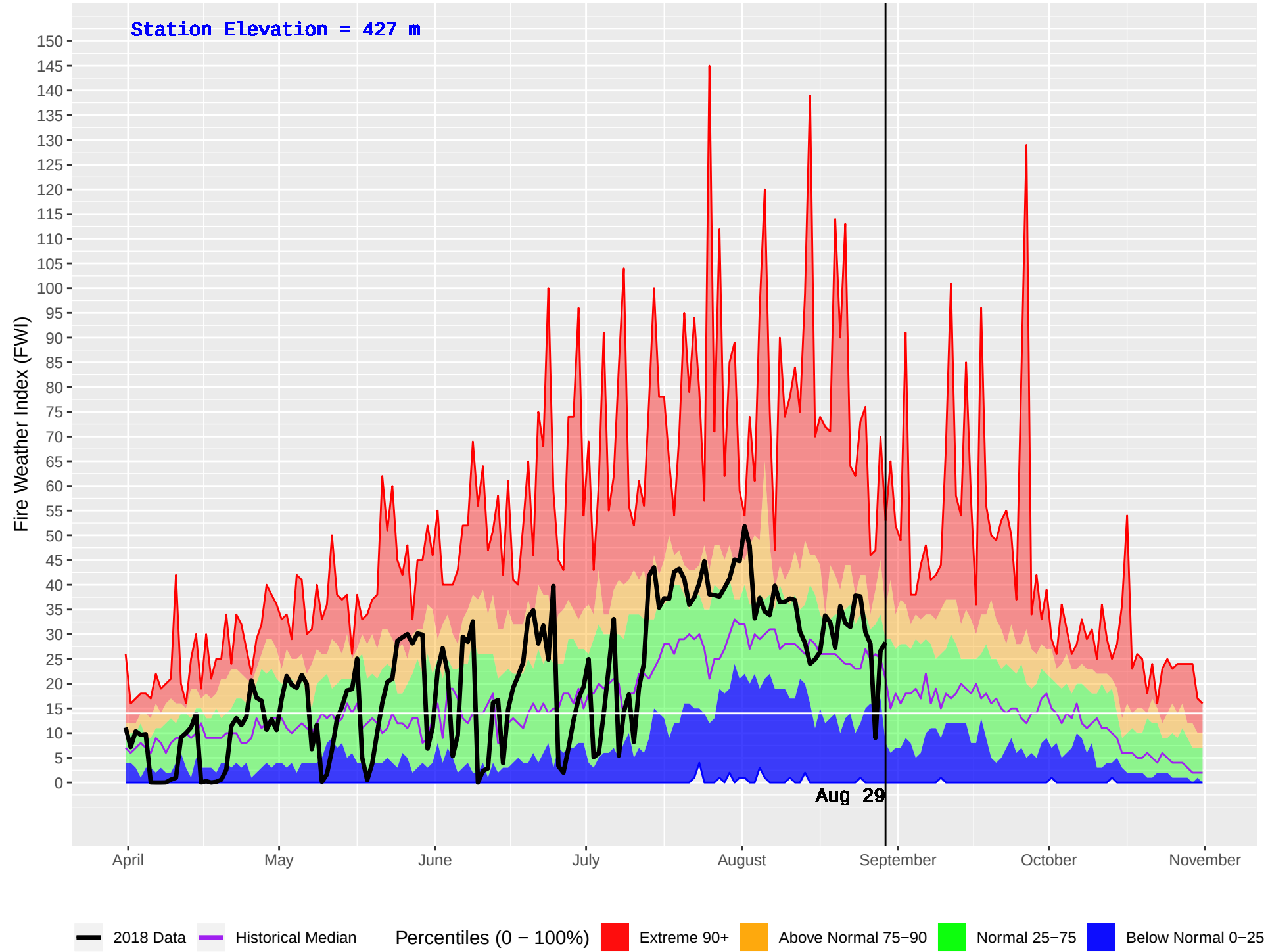
PENTICTON RS (328) : Historical (1970–2016) and Current (2018) Daily Fire Weather Index (FWI)
