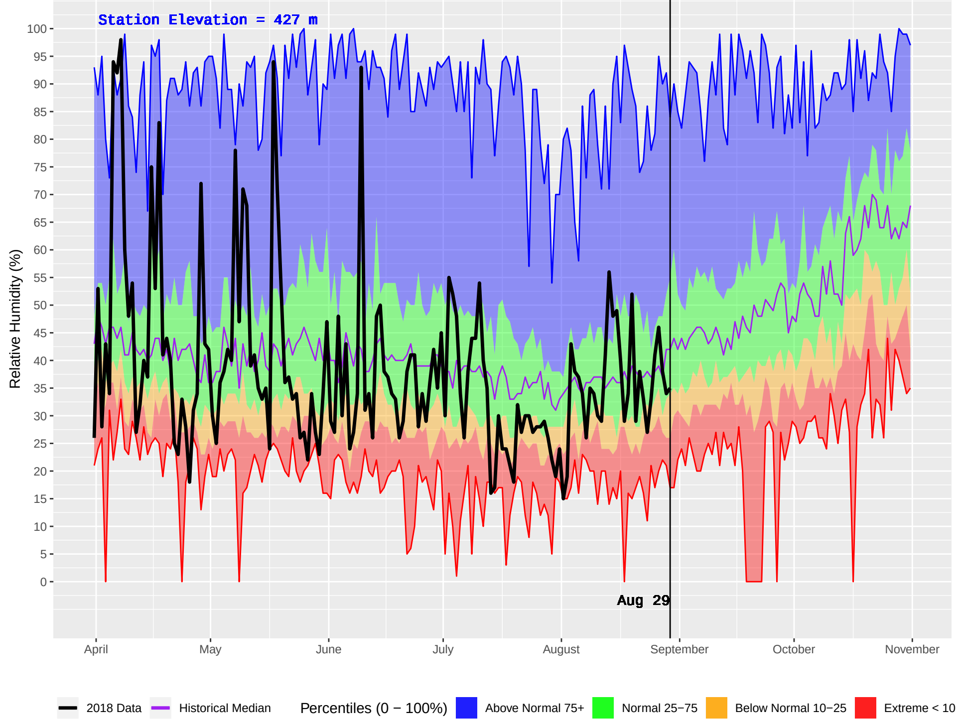
PENTICTON RS (328) : Historical (1970–2016) and Current (2018) Daily Relative Humidity
