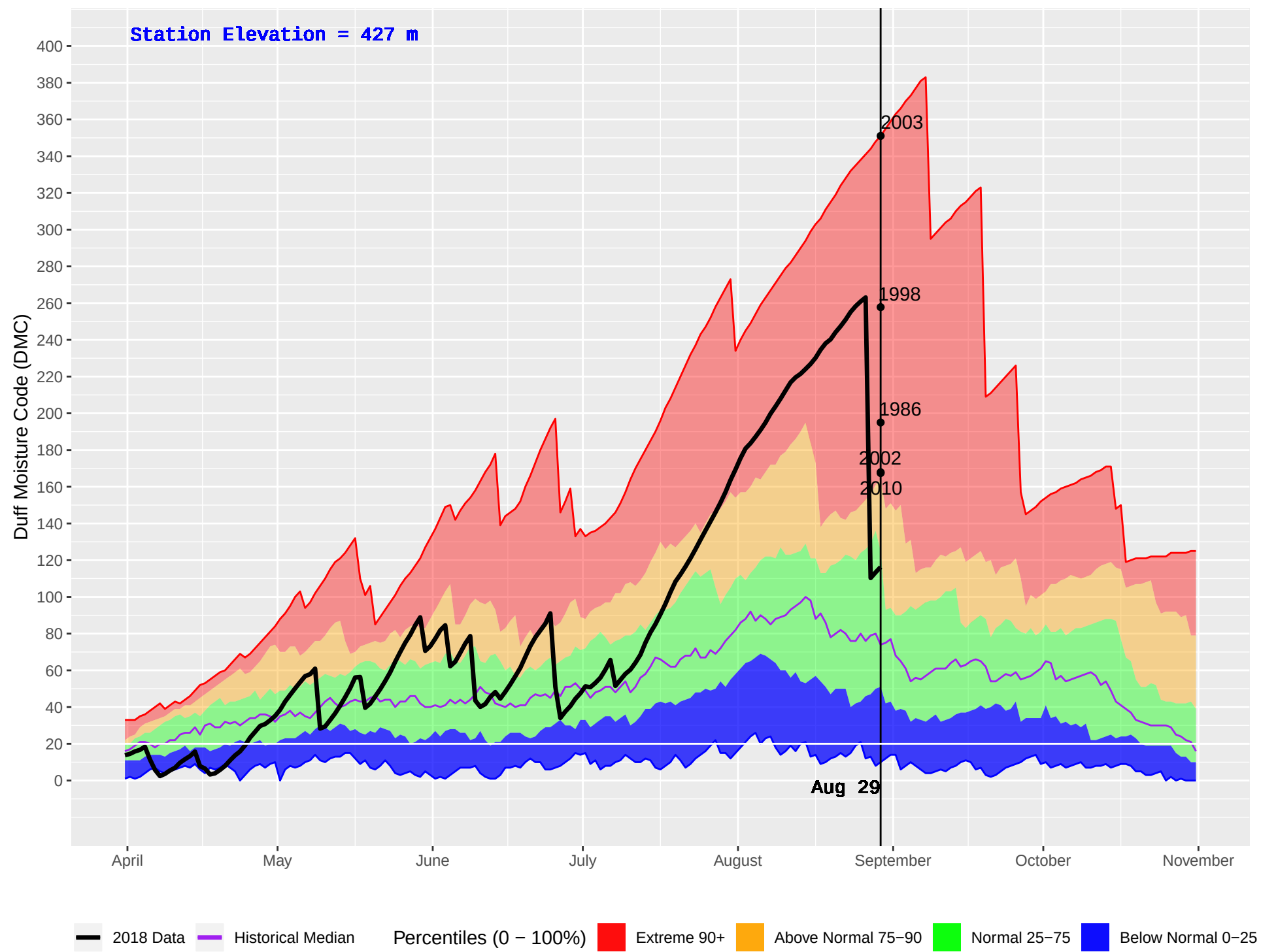
PENTICTON RS (328) : Historical (1970–2016) and Current (2018) Daily Duff Moisture Code (DMC)
